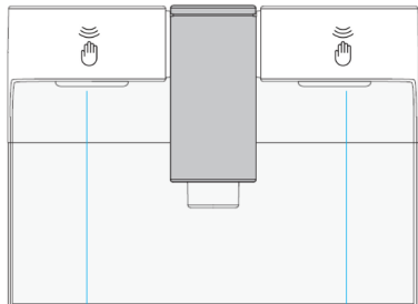
Infra Red Sensor for Cold water dispensing (Left side) Infra Red Sensor for ambient water dispensing (Right side)
